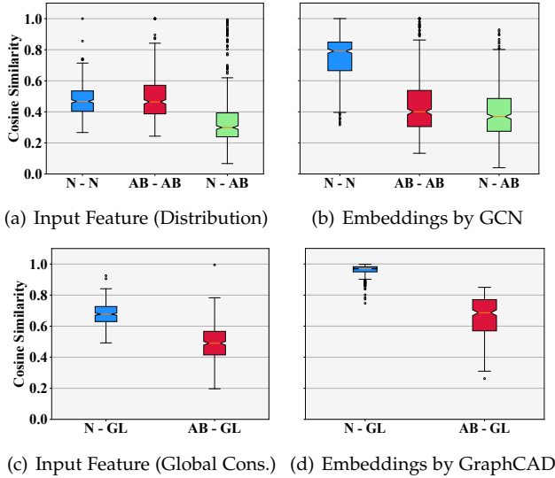
Fig. 2. (a) The similarities between normal and normal nodes (blue), abnormal and abnormal nodes (red), and normal and abnormal nodes (green) by the BERT-initialized input features; (b) The similarities between embeddings generated by GCN. (c) The similarities between normal nodes and the global context (blue) vs. those between abnormal nodes and the global context (red) by the input features; (d) The similarities between embeddings generated by GraphCAD.
